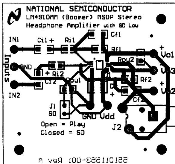
Figure 16. Composite View
