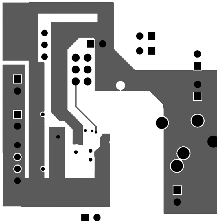
Figure 35. Signal 2 Layer
