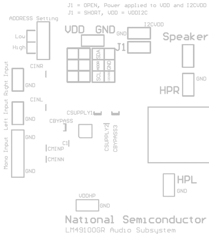
Figure 37. Top Overlay
