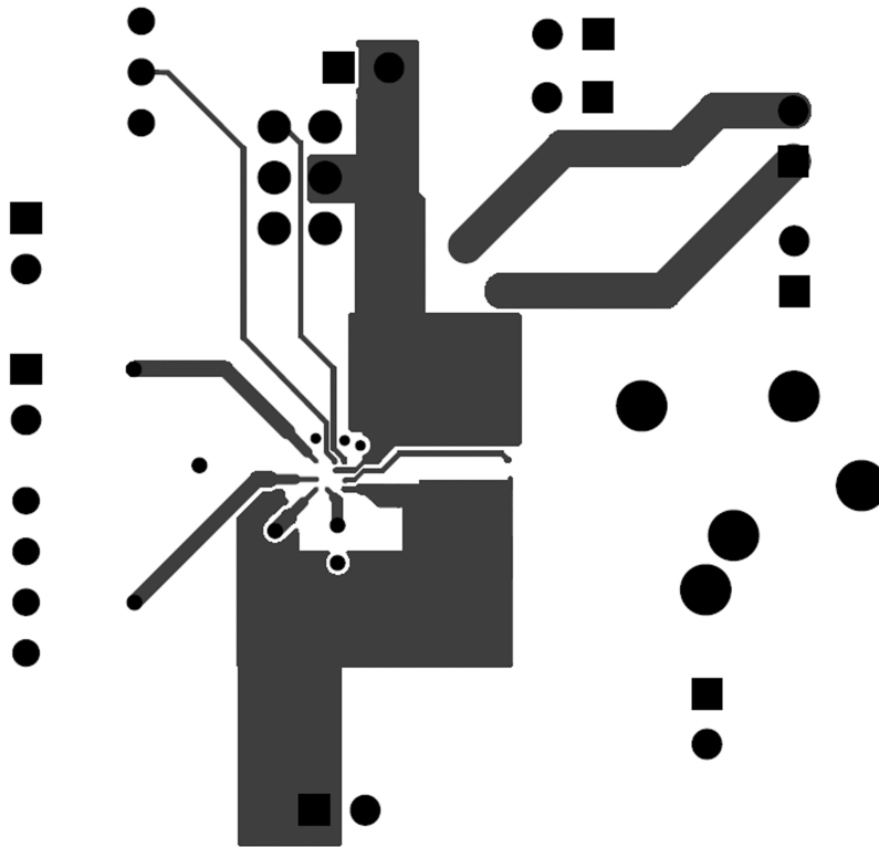
Figure 34. Signal 1 Layer
