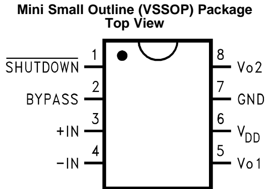
Figure 2. See Package Number DGK0008A
