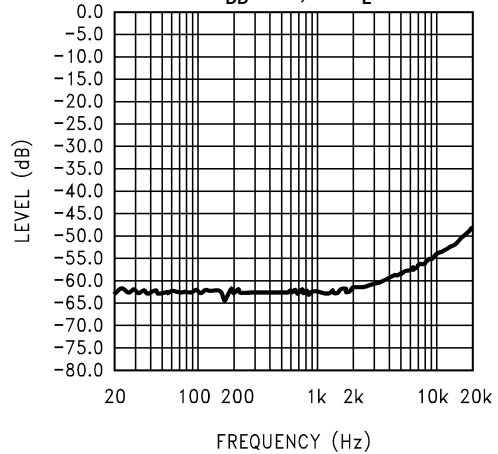
Figure 13. Input Floating
