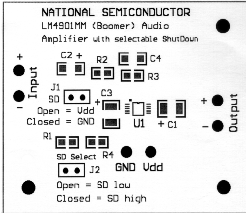
Silk Screen
