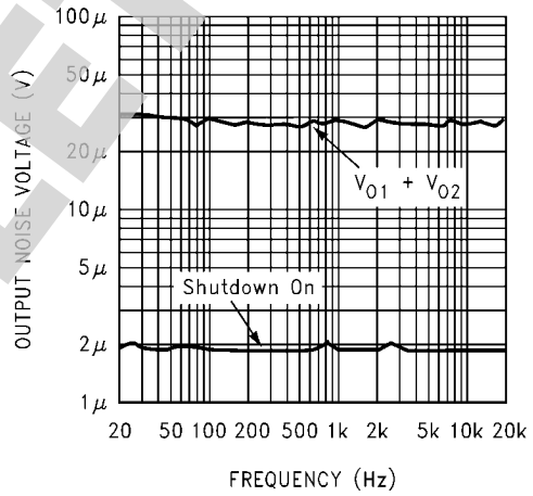
Noise Floor
