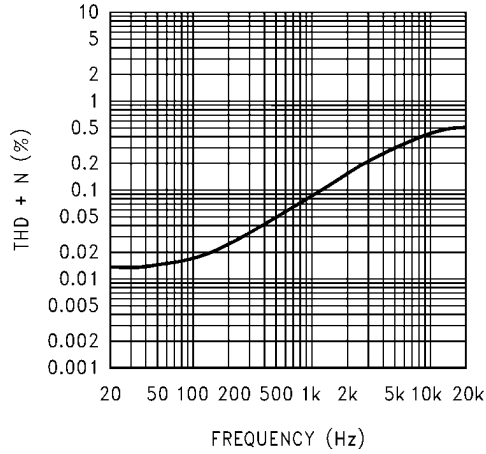
THD+N vs Frequency @ V_{DD} = 2.6V , 4\Omega R_L , and PWR = 150mW
