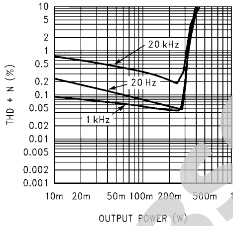
THD+N vs Output Power @ V_{DD} = 3V , 8\Omega R_L
