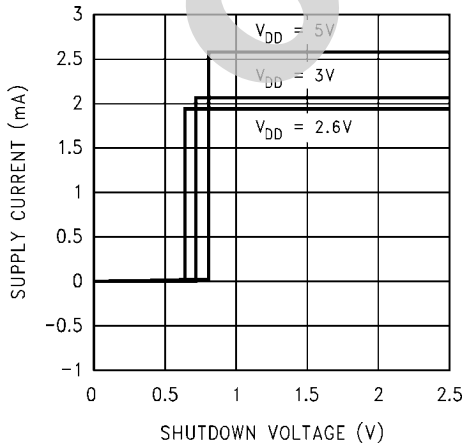
Supply Current vs Shutdown Voltage Shutdown Low
