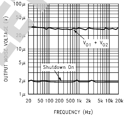
Noise Floor
