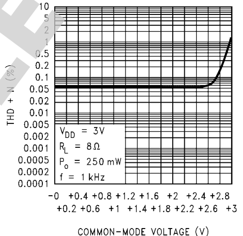
THD vs Common-Mode Voltage
