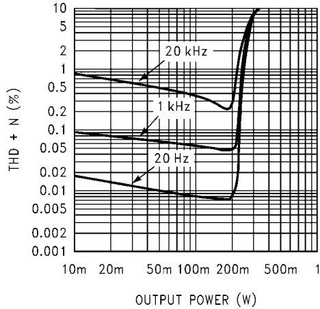
THD+N vs Output Power @ V_{DD} = 2.6V, 8\Omega R_L
