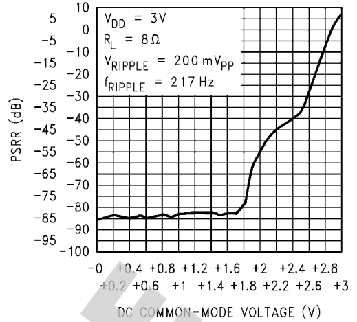
PSRR vs DC Common-Mode Voltage
