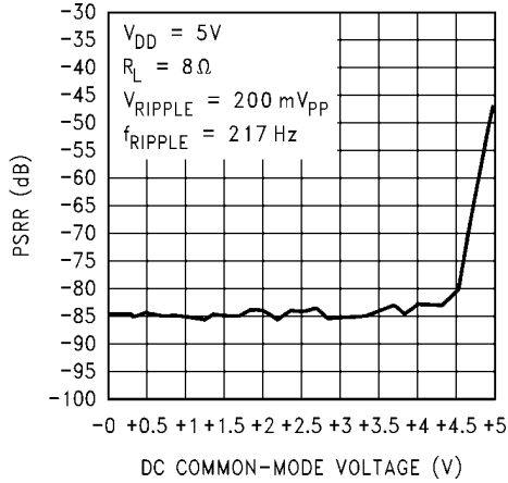
PSRR vs DC Common-Mode Voltage
