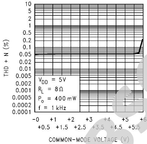
THD vs Common-Mode Voltage
