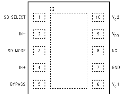
Top View Order Number LM4894LD See NS Package Number LDA10B
