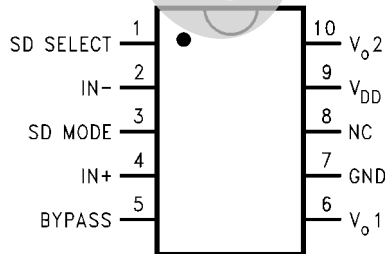
Top View Order Number LM4894MM See NS Package Number MUB10A
