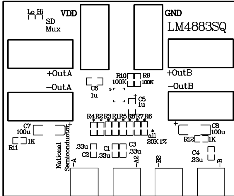
FIGURE 7. Silkscreen
