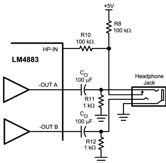
FIGURE 4. Headphone Circuit
