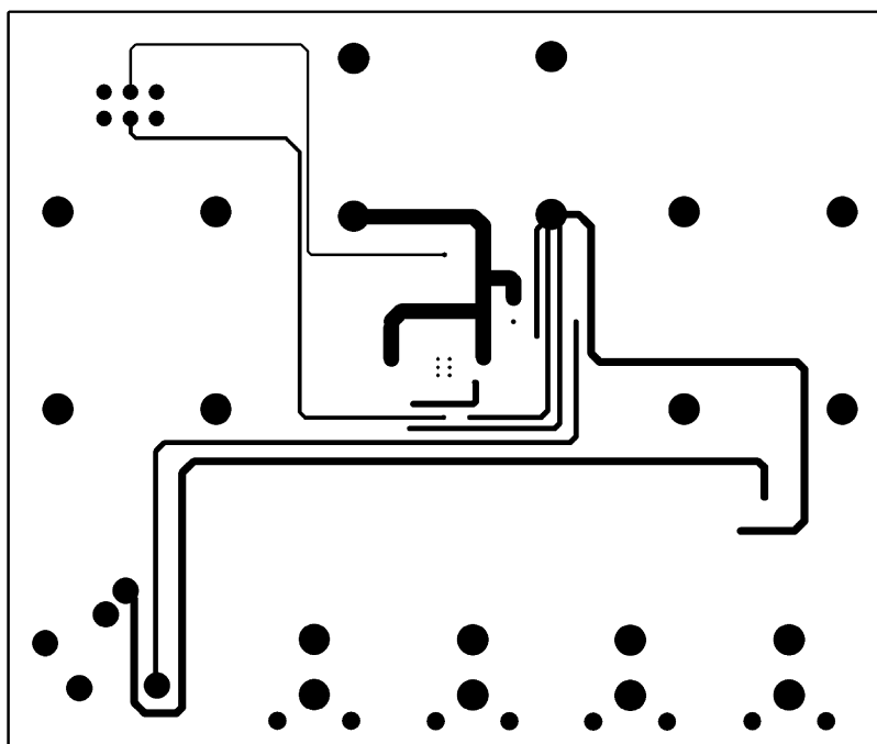
FIGURE 6. Bottom Layer
