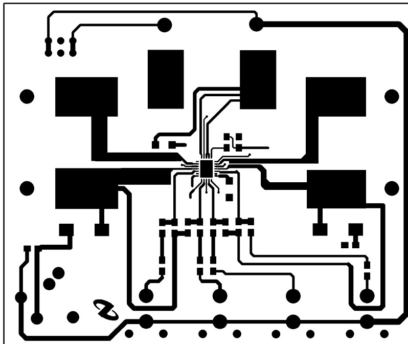
FIGURE 5. Top Layer
