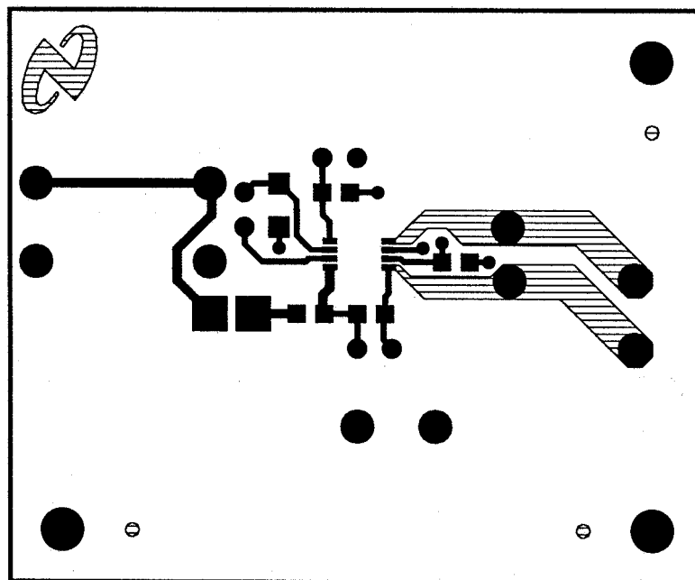
Figure 46. Top Layer
