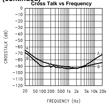
Figure 33. V_{DD} = 5V , R_L = 8\Omega , A_V = 10dB , A = Left channel driven, right channel measured; B = Right channel driven, left channel measured
