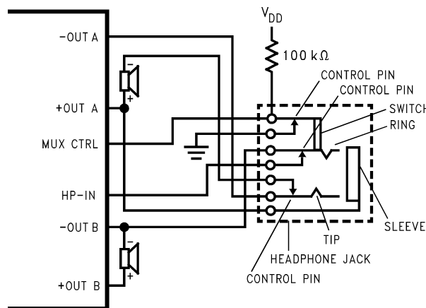
As configured, connecting headphones to this jack automatically selects the stereo headphone amplifier and, with the additional NC switch, changes MUX channels (Network 2 in Figure 43)
