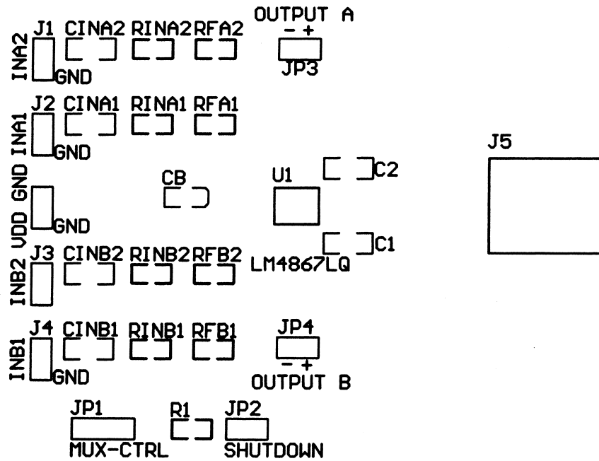
Figure 47. Recommended LQ PC Board Layout: Component-Side Silkscreen
