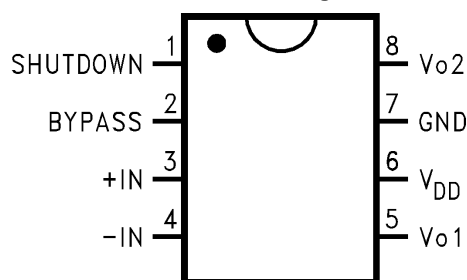
Connection Diagram
