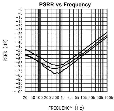
V_{DD} = 5V ; LLS, RLS; R_L = 8\Omega ; 0db Gain; All audio inputs terminated Top-Mode 12, 13; Mid-Mode 2, 3; Bot-Mode 7, 8
