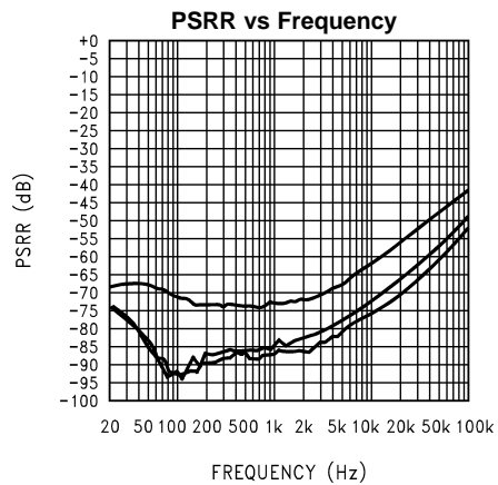
V_{DD} = 5V ; LHP, RHP; R_L = 32\Omega ; 0db Gain; All audio inputs terminated Top-Mode 13, 14; Mid-Mode 3, 4; Bot-Mode 8, 9
