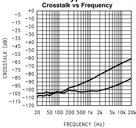
V_{DD} = 5V ; LLS, RLS; P_O = 400mW ; R_L = 8\Omega ; Mode 7; 0db Gain; 3D off Top-Left to Right; Bot-Right to Left Figure 20.
