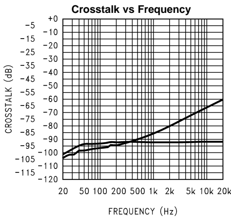
V_{DD} = 5V ; LHP, RHP; P_O = 15mW ; R_L = 32\Omega ; Mode 9; 0db Gain; 3D off Top-Left to Right; Bot-Right to Left Figure 22.
