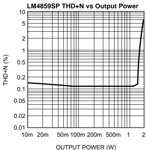
V_{DD} = 5V ; LLS, RLS; f = 1kHz ; R_L = 4\Omega ; Mode 7; 0dB Gain
