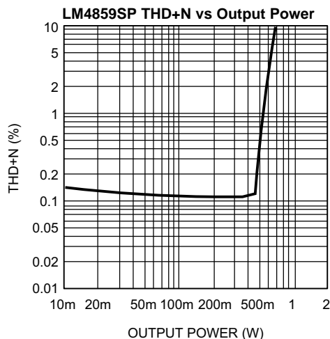
V_{DD} = 3V ; LLS, RLS; f = 1kHz ; R_L = 4\Omega ; Mode 7; 0dB Gain
