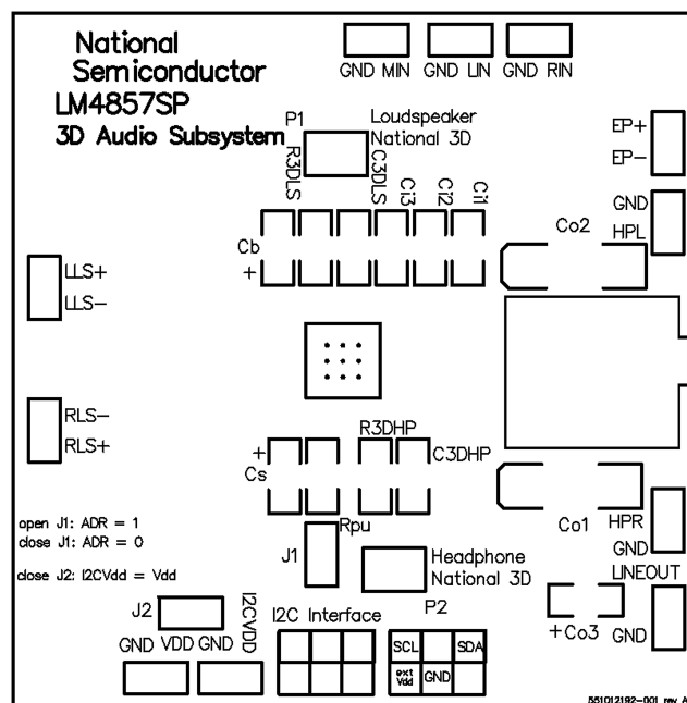
Figure 61. Recommended UQFN PCB Layout: Top Over Layer
