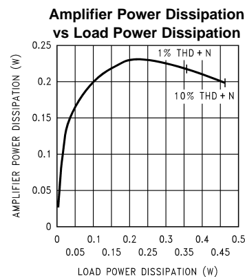
Figure 37. LM4854IBL/MT, V_{DD} = 3V , R_L = 8\Omega (BTL), f_{IN} = 1kHz
