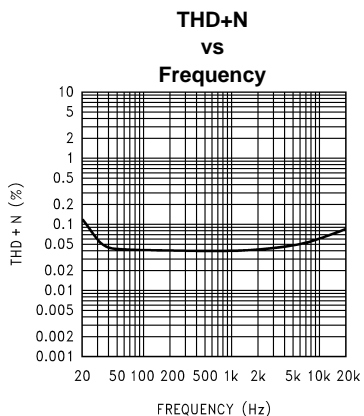
Figure 12. V_{DD} = 5V , R_L = 32\Omega (SE), P_{OUT} = 50mW
