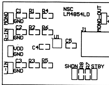
Figure 59. Recommended LD PC Board Layout: Component-Side SilkScreen
