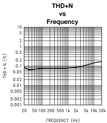
Figure 10. V_{DD} = 5V , R_L = 8\Omega (BTL), P_{OUT} = 400mW
