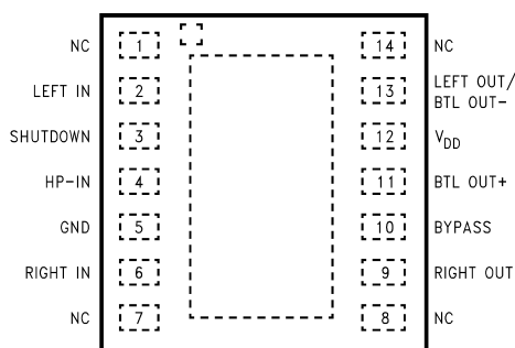
Figure 2. 14 Lead WSON – Top View See Package Number NHE0014A
