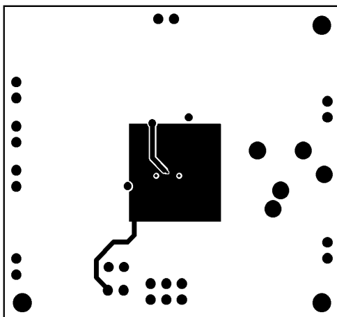
Figure 40. Recommended ITL PC Board Layout: Middle 1 Layer
