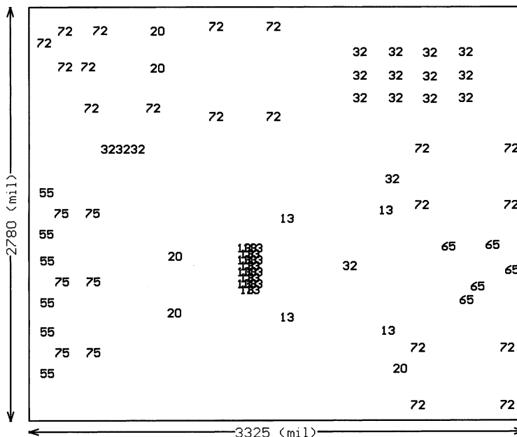
Figure 61. Drill Drawing
