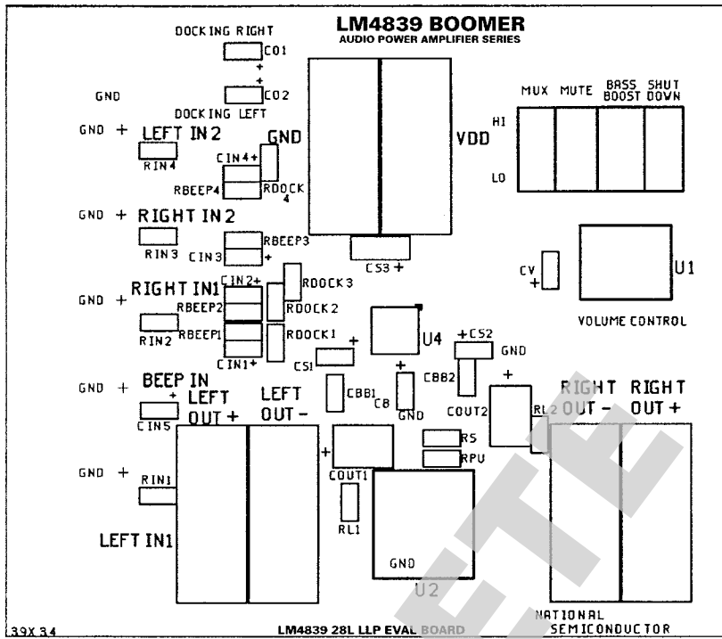
LM4839 28L LLP EVAL BOARD NATIONAL SEMICONDUCTOR
