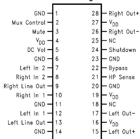
TSSOP Package
