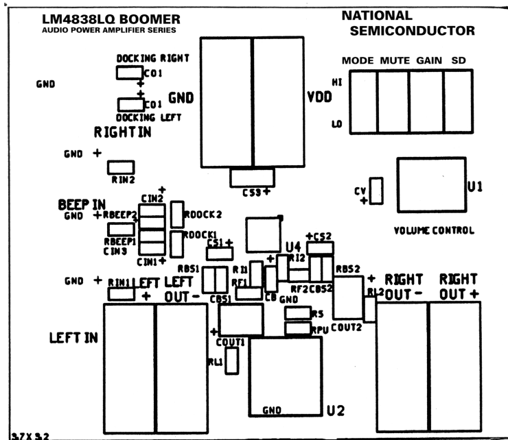
Figure 57. Recommended NJB PC Board Layout: Component-Side Silkscreen
