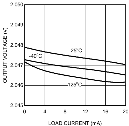
Figure 18. Load Regulation
