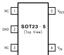
Figure 1. SOT23-5 Surface Mount Package
