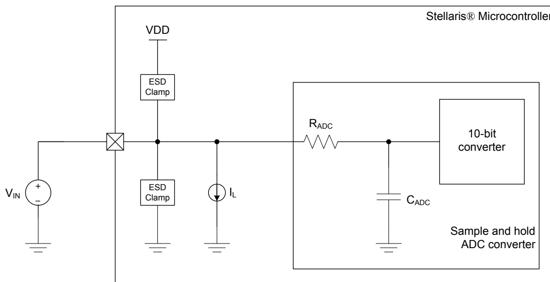
Figure 26-12. ADC Input Equivalency Diagram
