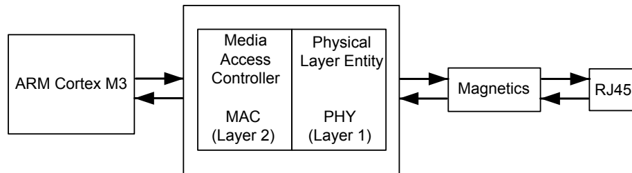
Figure 19-1. Ethernet Controller
