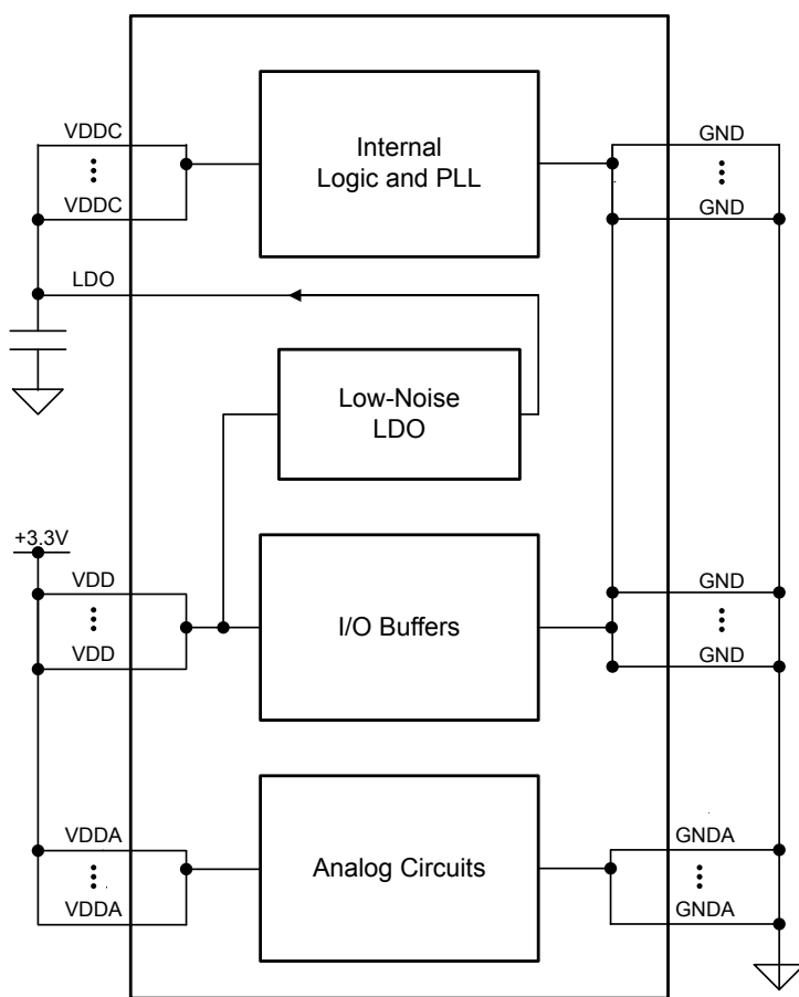
Figure 5-4. Power Architecture
