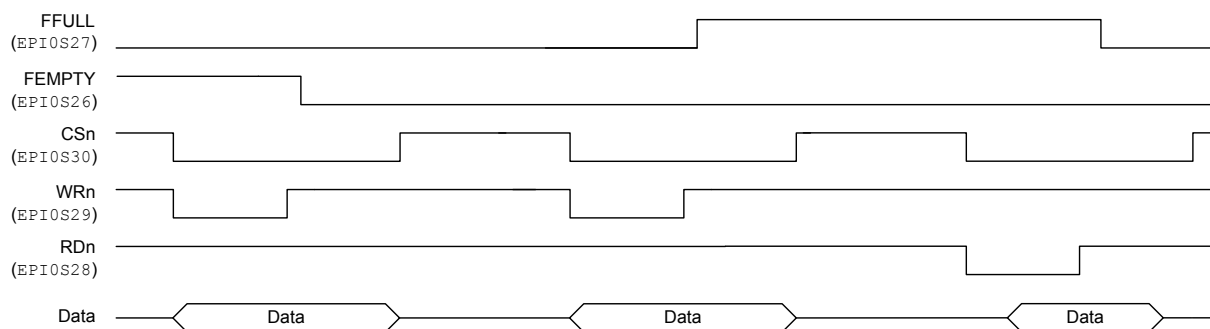
Figure 9-10. Two-Entry FIFO
