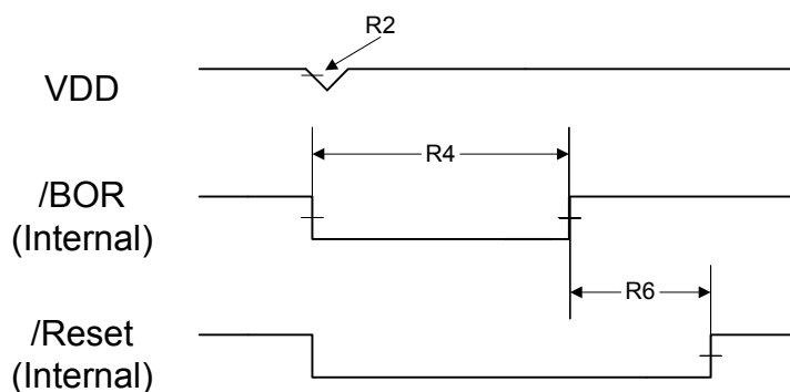
Figure 26-7. Brown-Out Reset Timing
