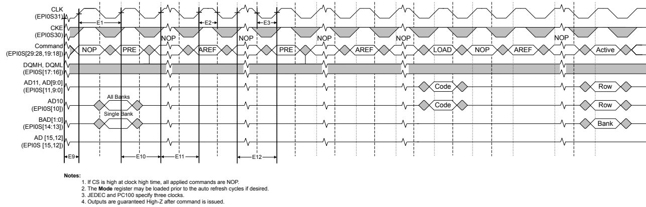
Figure 25-14. SDRAM Initialization and Load Mode Register Timing
