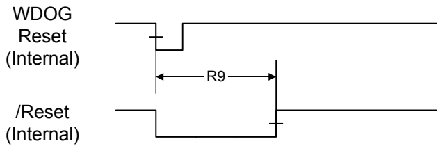
Figure 17-9. Watchdog Reset Timing
