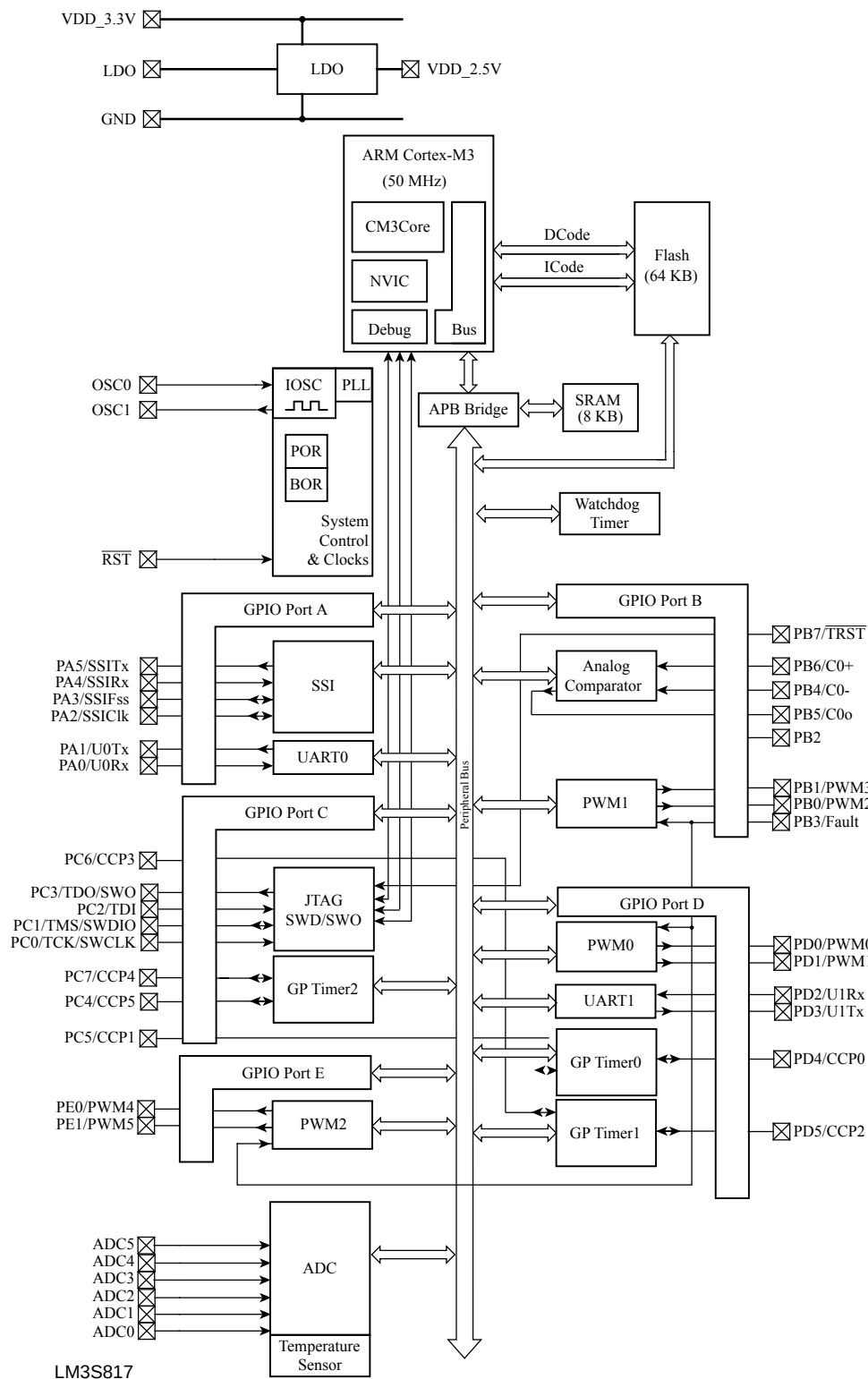
Figure 1-2. LM3S817 Controller System-Level Block Diagram
