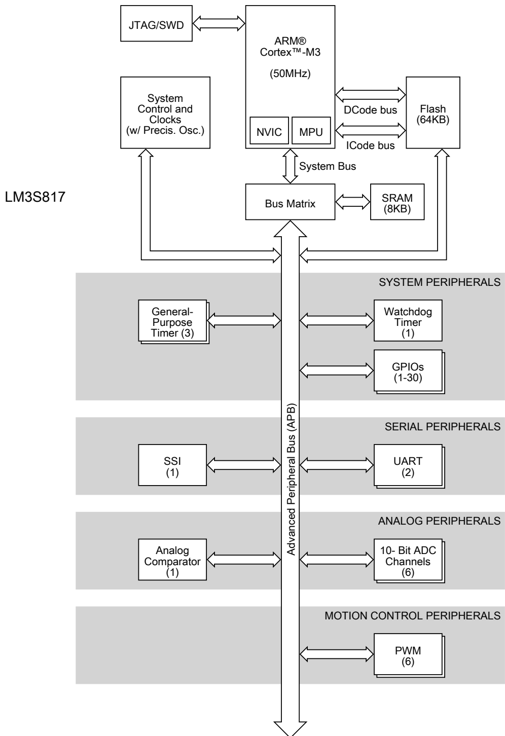
Figure 1-1. Stellaris LM3S817 Microcontroller High-Level Block Diagram
