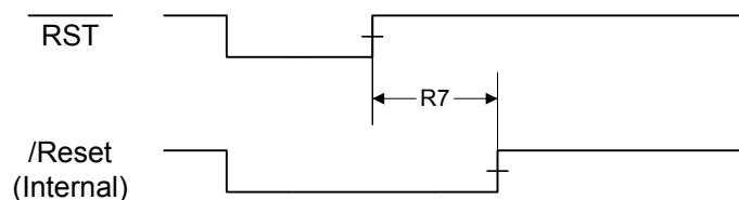
Figure 19-5. External Reset Timing (RST)
