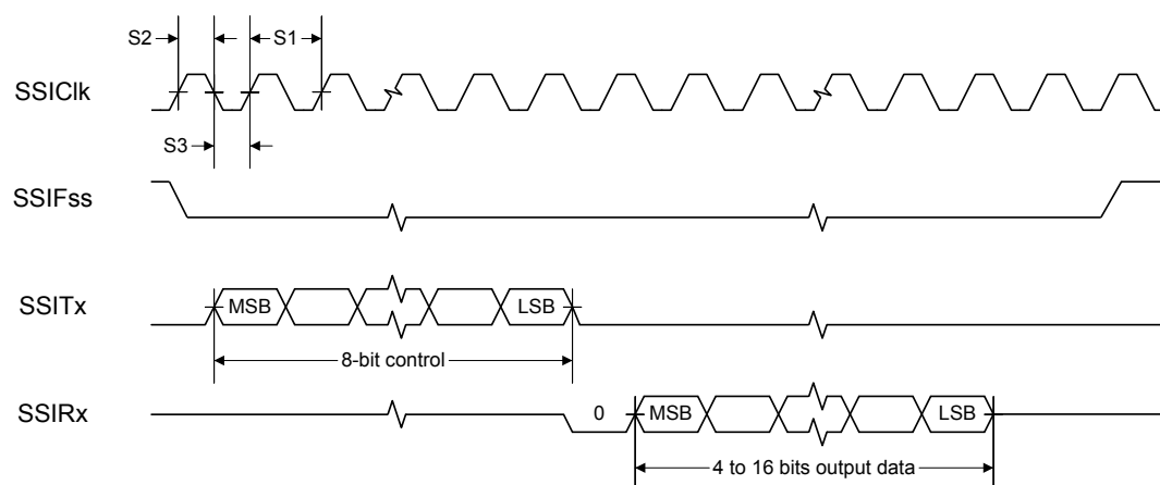
Figure 25-19. SSI Timing for MICROWIRE Frame Format (FRF=10), Single Transfer
