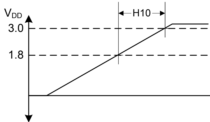
Figure 25-16. VDD Ramp when Waking from Hibernation
