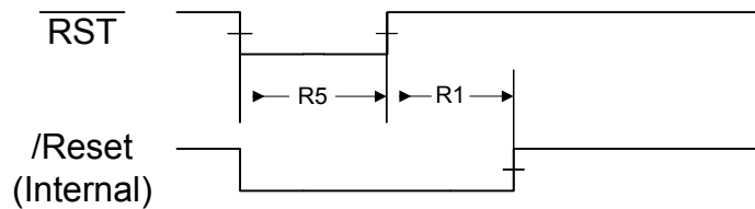
Figure 25-10. External Reset Timing ( \overline{\text{RST}} )
