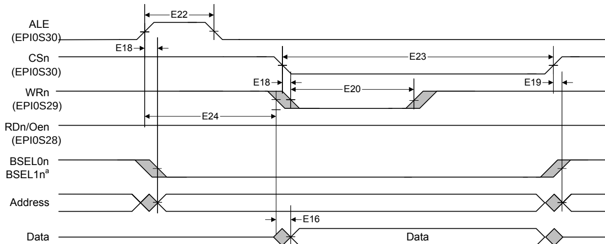
Figure 25-18. Host-Bus 8/16 Mode Write Timing
