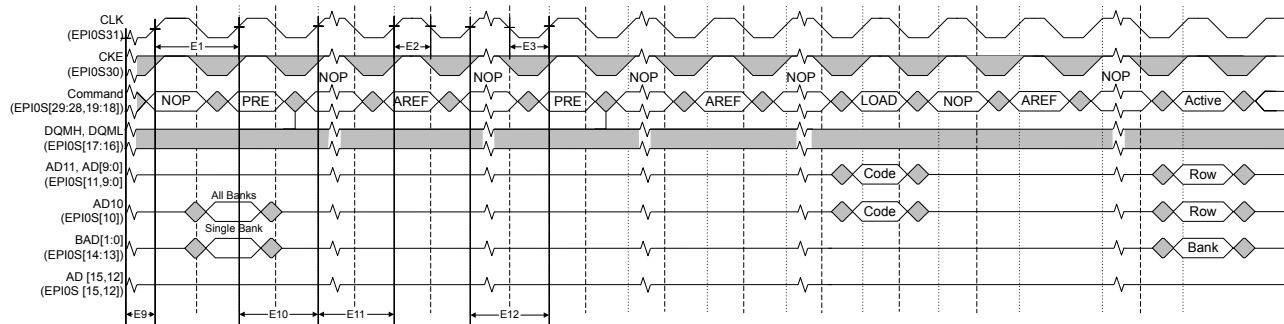
Figure 25-14. SDRAM Initialization and Load Mode Register Timing
