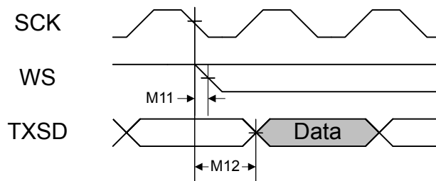
Figure 25-22. I 2 S Master Mode Transmit Timing
