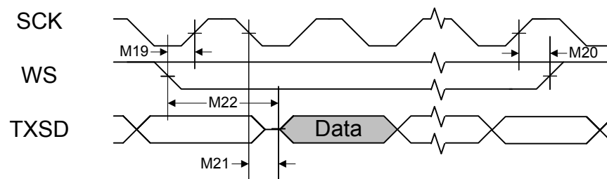
Figure 23-20. I 2 S Slave Mode Transmit Timing
