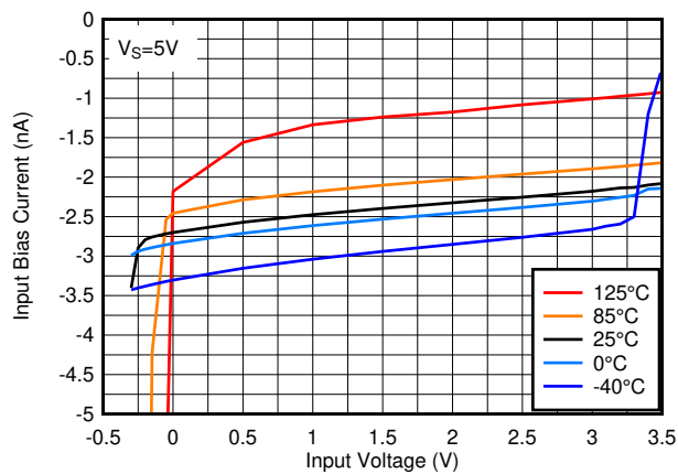
Figure 6-21. Input Bias Current vs. Input Voltage at 5\text{ V}
