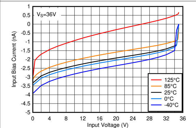
Figure 6-23. Input Bias Current vs. Input Voltage at 36V
