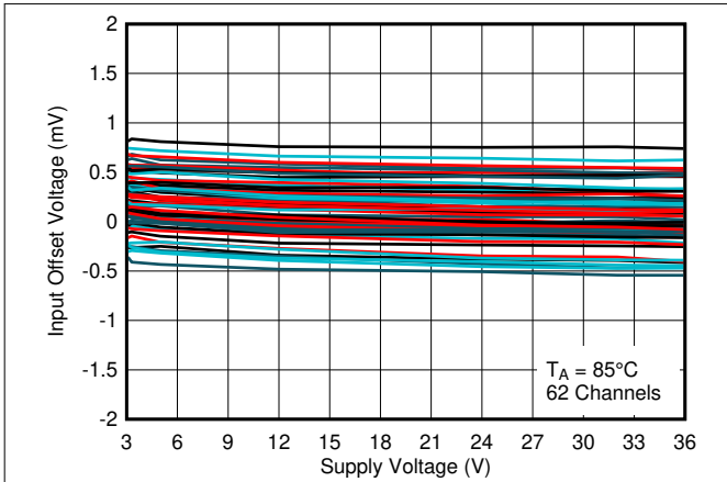
Figure 6-18. Input Offset Voltage vs. Supply Voltage at 85°C
