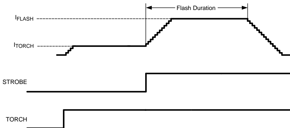
Figure 26. Hardware-Torch Mode
