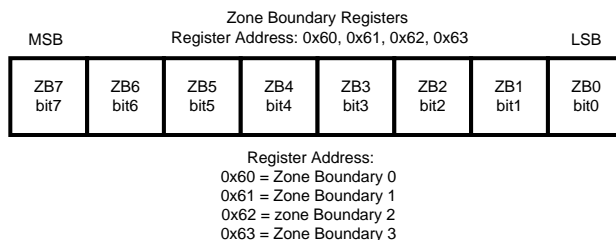
Figure 27. Zone Boundary Register Descriptions
