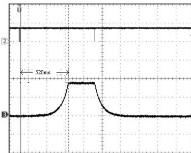
Channel 2: SDA (5V/div) Time Base (200ms/div) Channel 3: I_{LED} (10mA/div) 4.096ms/Step Up And Down
