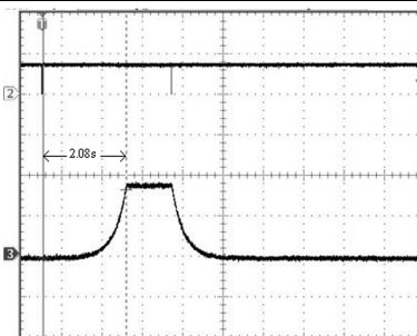
Channel 2: SDA (5V/div) Time Base (1s/div) Channel 3: I_{LED} (10mA/div) 16.384ms/Step Up And Down
