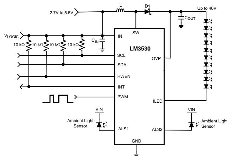
Figure 49. LM3530 Typical Application
