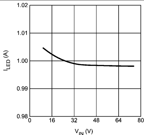
Figure 4. Buck-Boost LED Current vs. Input Voltage V_O = 21\text{ V} (6 LEDs)
