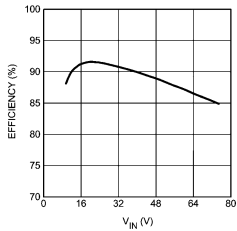
Figure 37. Sample Buck-Boost Efficiency vs Input Voltage. Vo = 21 V
