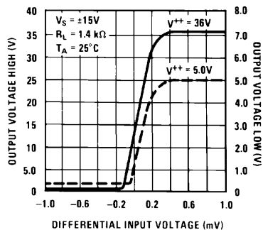
Figure 15. Transfer Function
