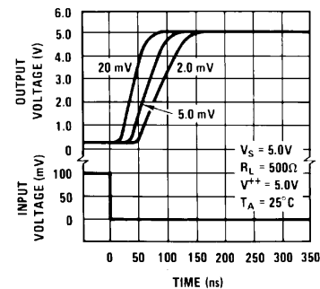
Figure 8. Response Time for Various Input Overdrives
