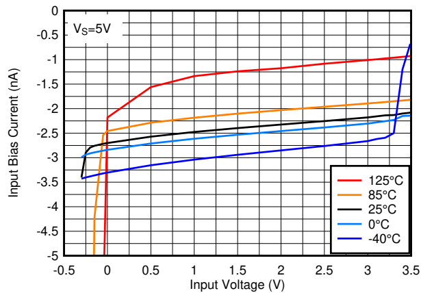
Figure 3-22. Input Bias Current vs. Input Voltage at 5\text{ V}
