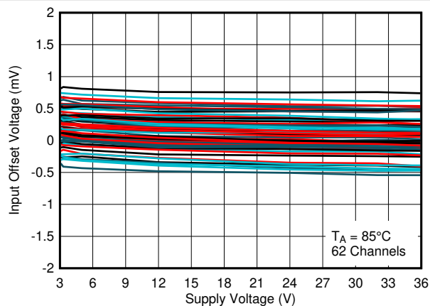
Figure 3-19. Input Offset Voltage vs. Supply Voltage at 85^\circ\text{C}
