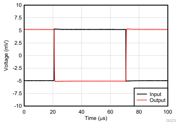
Figure 6-28. Overload Recovery
