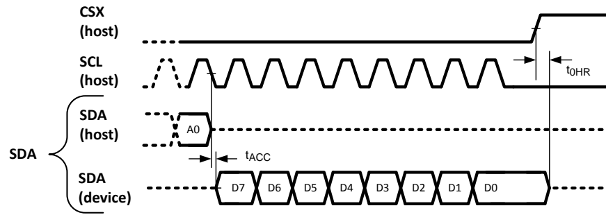
Figure 5. SPI Interface
