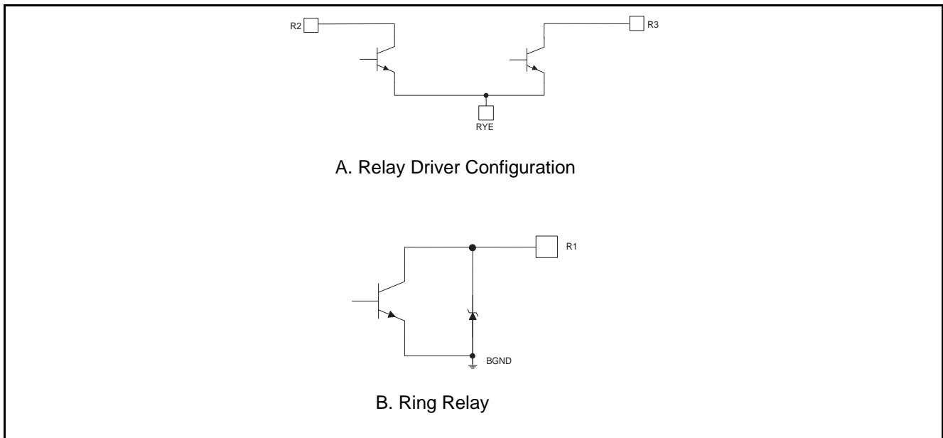
Figure 6 - Relay Drivers
