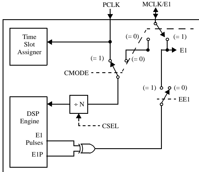
Figure 20 - Clock Mode Options (PCM/MPI Mode)
