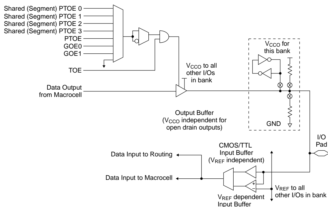
Figure 8. I/O Cell
